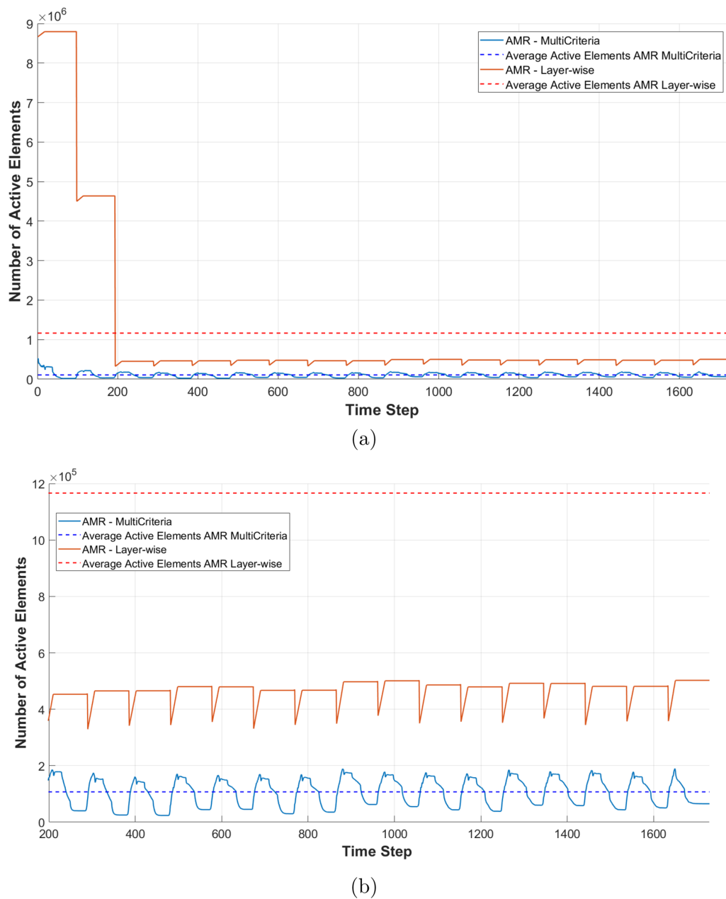
Fig. 21 Thin-wall: a evolution of the number of active FEs per time step; b detail from time-step 200 to the end of simulation for the 10 (min) waiting time case
