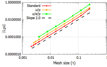
Fig. 4. Convergence rate of the displacement field of the three FE technologies upon mesh refinement.
