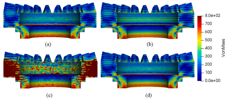
Fig. 19. Gear: Von-Mises stress at a cut along the central plane. (a) Fixed coarse mesh. (b) Fixed Fine mesh. (c) Adaptive mesh without correction terms. (c) Adaptive mesh with correction terms.
