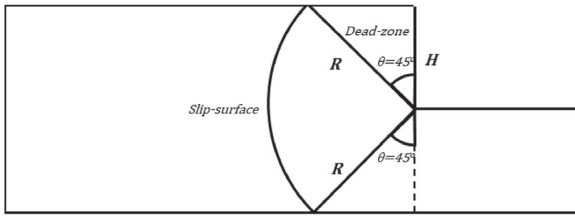
Fig. 19. Elasto-plastic extrusion with 2:1 reduction.
