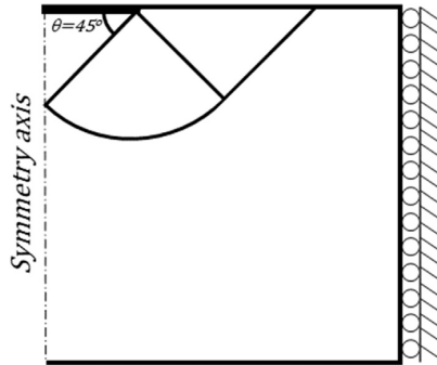
Fig. 26. Prandtl's Punch test: Collapse mechanism in an isothermal setting.
