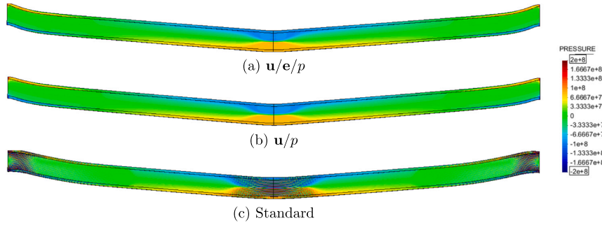
Fig. 9. Double clamped I-shaped beam: Pressure in [Pa].
