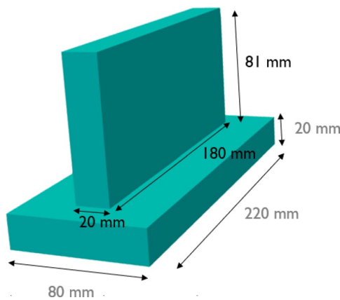
Fig. 17 Thin-wall: geometry
