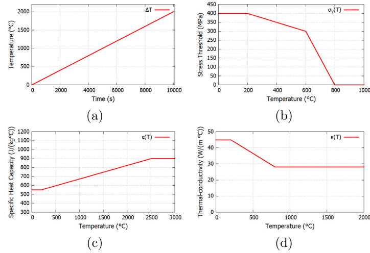
Fig. 21. 3D frame: (a) Heat source increment over time, (b) Uniaxial stress threshold, (c) Specific heat capacity, (d) Thermal conductivity, evolution with the temperature.
