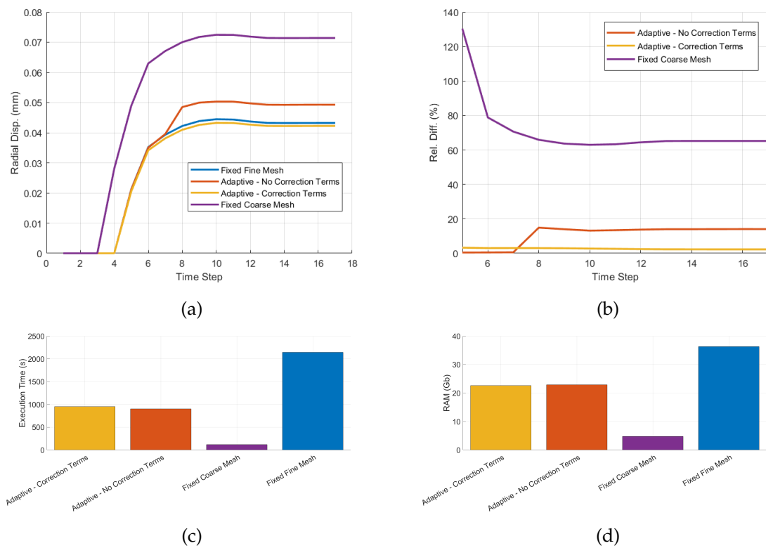
Figure 29: Coarsening correction terms influence on: (a) the displacement solution; (b) the relative percentual difference with respect to the reference solution; (c) simulation run times and (d) memory consumption.
