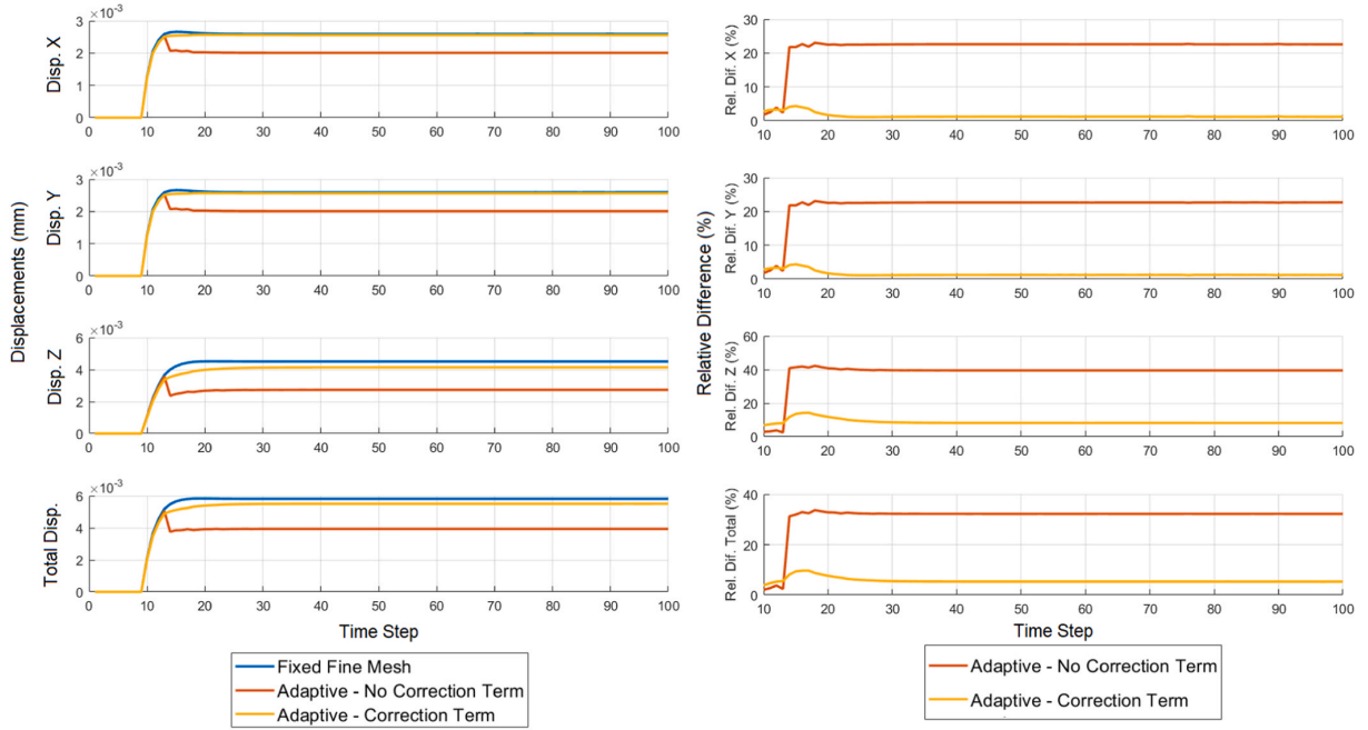
Fig. 11. Slender column: Evolution of the displacements (left) and the relative difference vs. the fixed fine mesh (right) at point P during the activation process.
