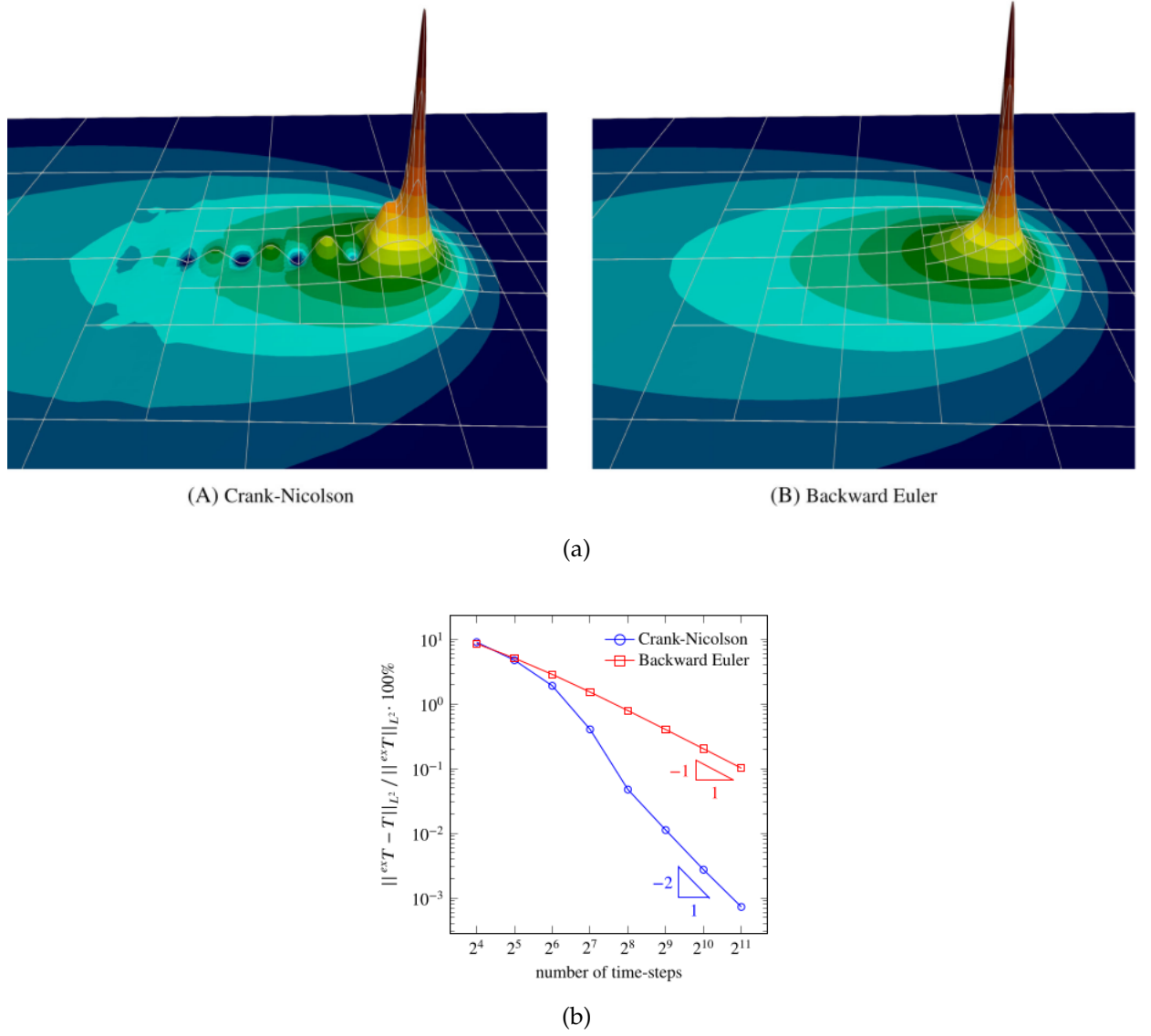
Figure 20: Comparative results between the backward Euler and the Crank-Nicholson methods. (a) Solution oscillations in the Crank-Nicholson results. (b) Convergence-rate of the time integration methods. (Kollmannsberger and Kopp, 2021)
