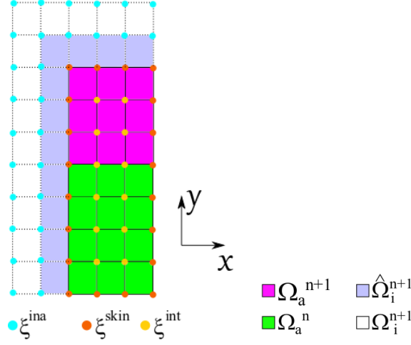
Figure 36: Definition of the evolving active domain ( \Omega_{act}^{n+1} \subseteq (\Omega_a^{n+1} \cup \Omega_a^n) ) and inactive domain ( \Omega_{ina}^{n+1} \subseteq (\Omega_i^{n+1} \cup \hat{\Omega}_i^{n+1}) ) and the node classification.
