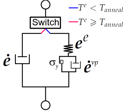
Figure 21: Phase-change model according to the FE temperature.
