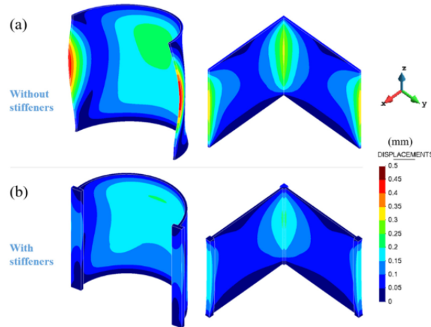
Figure 9: Open thin-walled structures warpage: (a)-(b) without and with vertical stiffeners, respectively. (Lu et al., 2021c).
