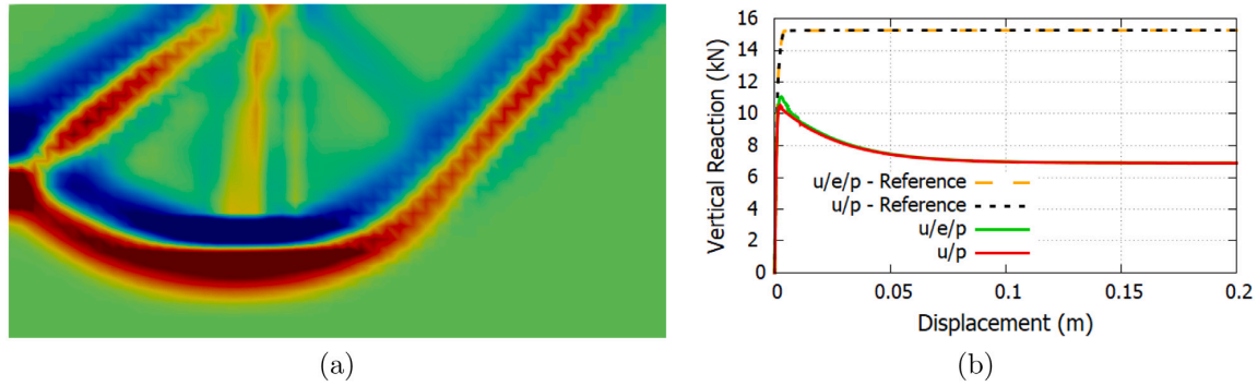
Fig. 30. Prandtl's Punch test — case 2: (a) Superimposed collapse mechanisms at d_p = 0.20 [m]. In red the u/e/p solution and the u/p in blue; (b) Reaction vs displacement curves. (For interpretation of the references to colour in this figure legend, the reader is referred to the web version of this article.)
