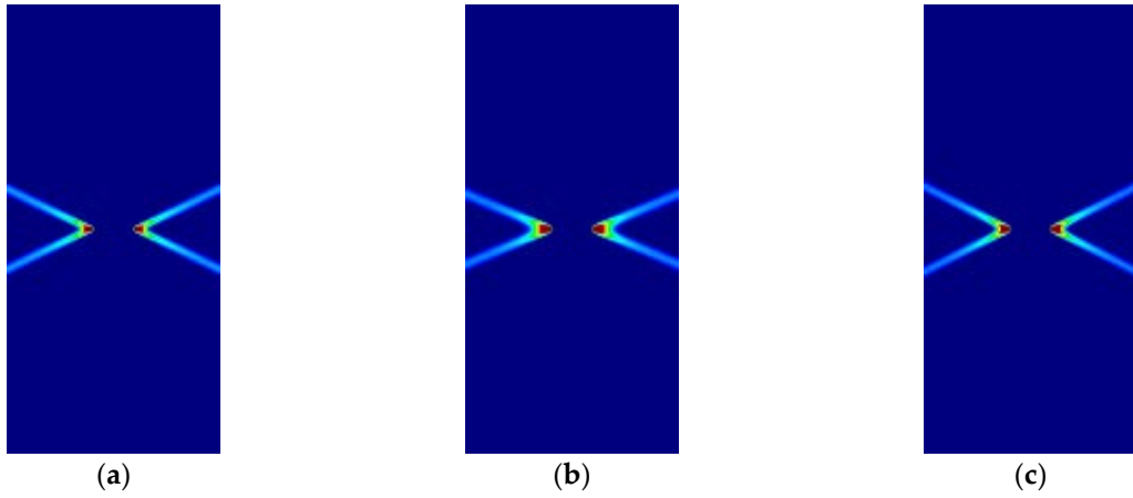
Figure 11. Strip under vertical plane stress tension (Cohesive-frictional models, \kappa = 1.5 ): (a) Parabolic Drucker-Prager; (b) Hoffman; (c) Tsai-Wu.
