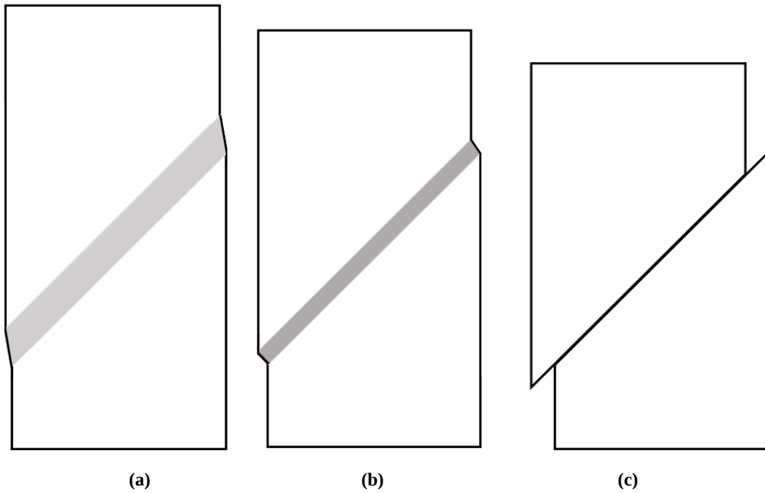
Figure 3.1 Stages of failure: (a) continuous failure, (b) localized failure and (c) discrete failure
