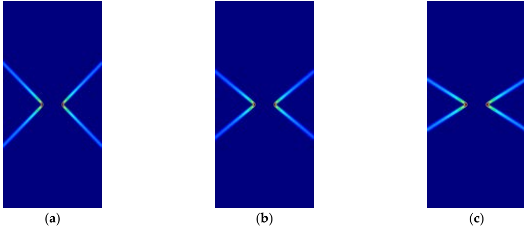
Figure 9. Strip under vertical plane strain tension (Parabolic Drucker-Prager): (a) \kappa = 1 identical to von-Mises; (b) \kappa = 1.25 ; (c) \kappa = 1.5 .
