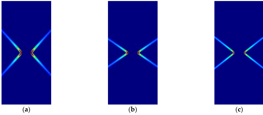
Figure 12. Strip under vertical plane stress compression (Cohesive-frictional models, \kappa = 3.0 ): (a) Parabolic Drucker-Prager; (b) Hoffman; (c) Tsai-Wu.
