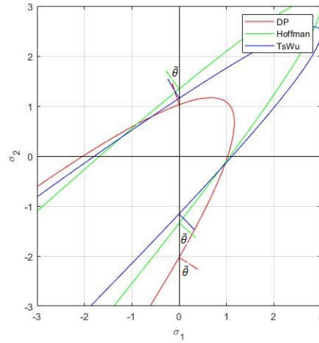
(b) Plane Strain with \kappa = 1.5
