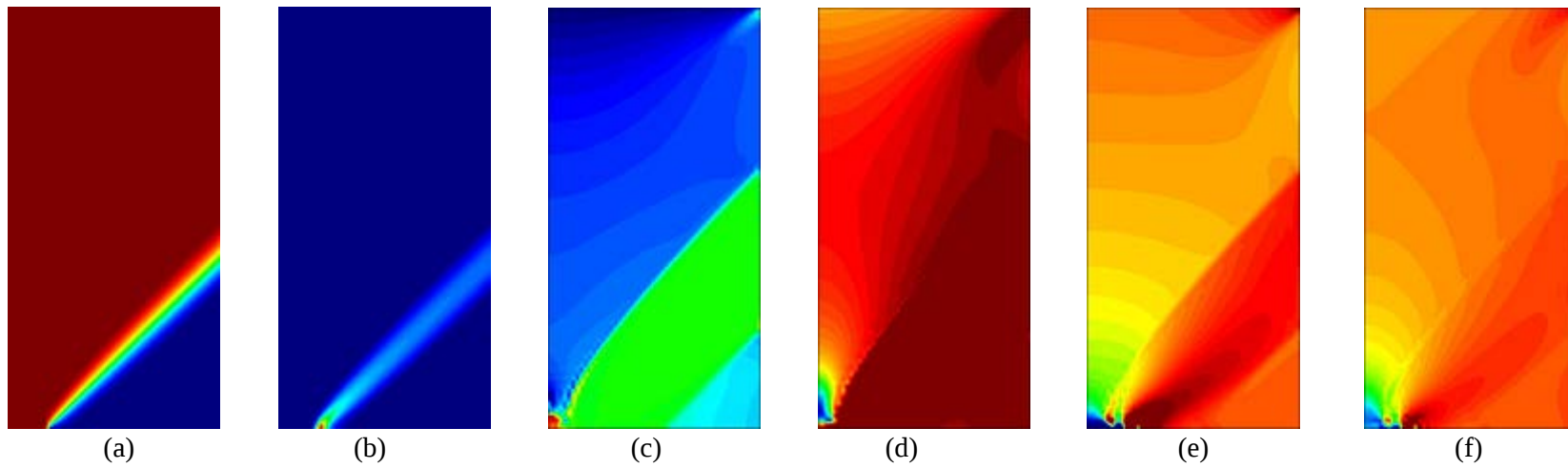
Figure 4.11 Contour fills for quads mixed \varepsilon/\bar{B} -bar u FE, von Mises: (a) Y-disp, (b) Equiv. plast. strain, (c) Lode angle, (d) J_2 stress, (e) Mean stress, (f) Y-stress
