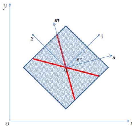
282 Figure 4. Definition of the localization angle \theta_{cr} .
