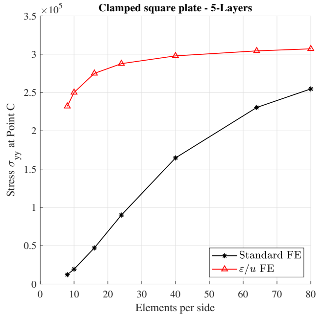
Fig. 38: Clamped square plate with five layers of orthotropic materials: Normal stress \sigma_{yy} at Point C on the top surface of the plate (see Fig. 17) versus number of finite elements per side.
