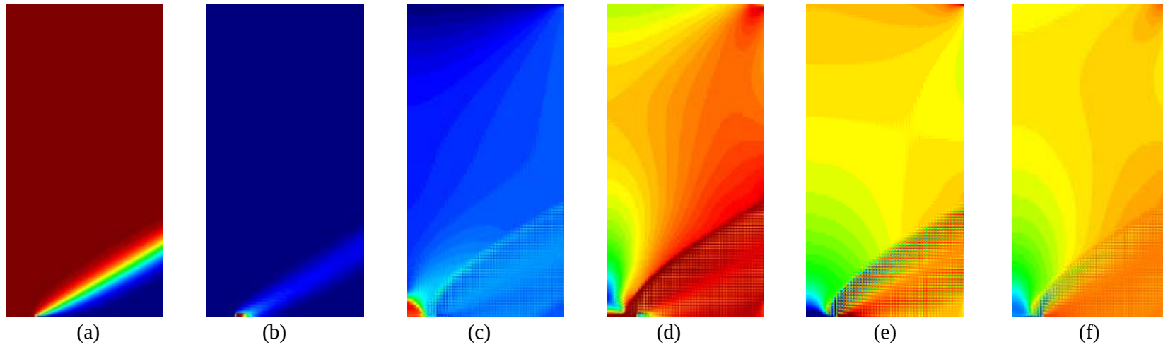
Figure 4.13 Contour fills for quads irreducible u FE, Drucker-Prager: (a) Y-disp, (b) Equiv. plast. strain, (c) Lode angle, (d) J_2 stress, (e) Mean stress, (f) Y-stress
