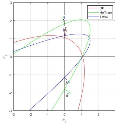
(d) Plane Strain with \kappa = 3.0
