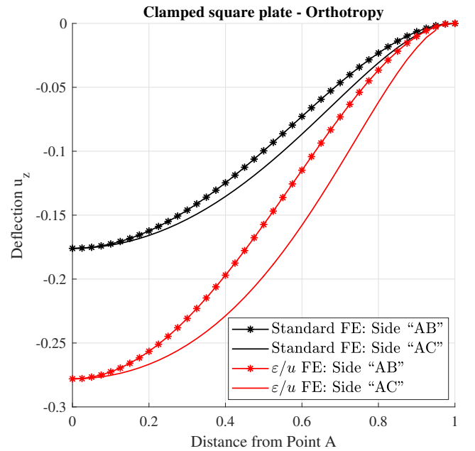
Fig. 31: Clamped square plate with orthotropy: Deflection u_z along two two midsides “AB” and “BC” (see Fig. 17).
