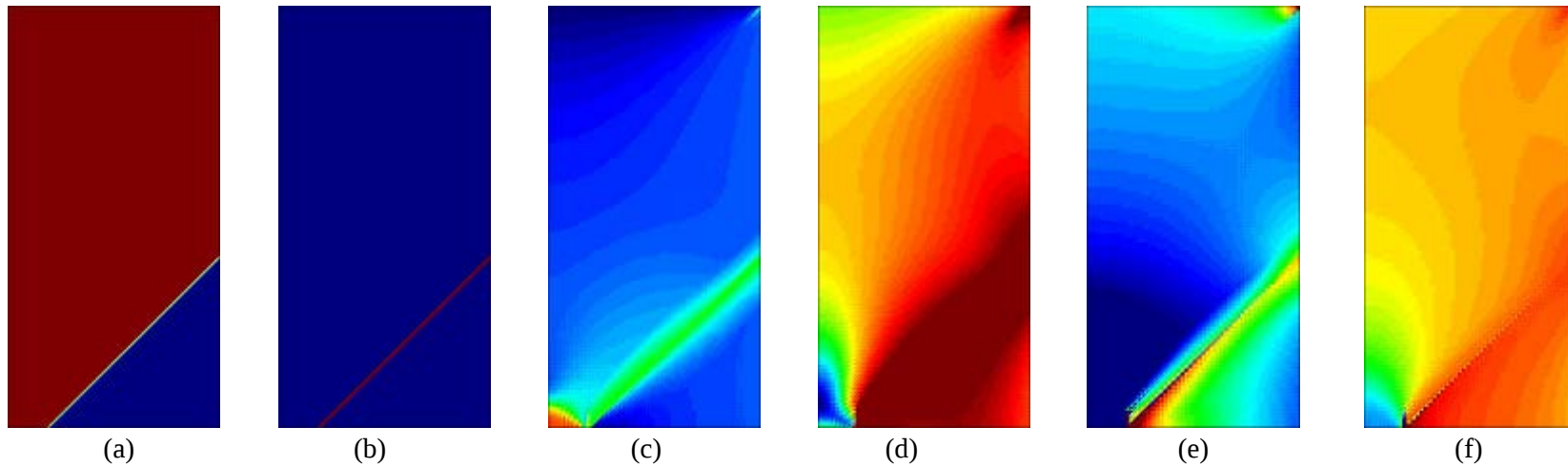
Figure 4.3 Contour fills for triangular irreducible u FE, von Mises: (a) Y-disp, (b) Equiv. plast. strain, (c) Lode angle, (d) J_2 stress, (e) Mean stress, (f) Y-stress
