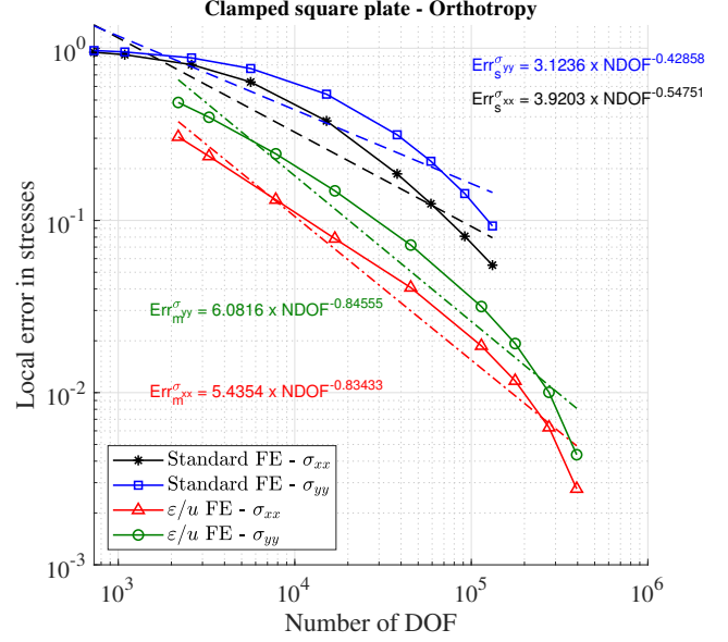
Fig. 30: Clamped square plate with orthotropy: Local error in the stresses \sigma_{xx} , \sigma_{yy} at Points B and C (see Fig. 17) versus the Number of Degrees of Freedom (DOF).
