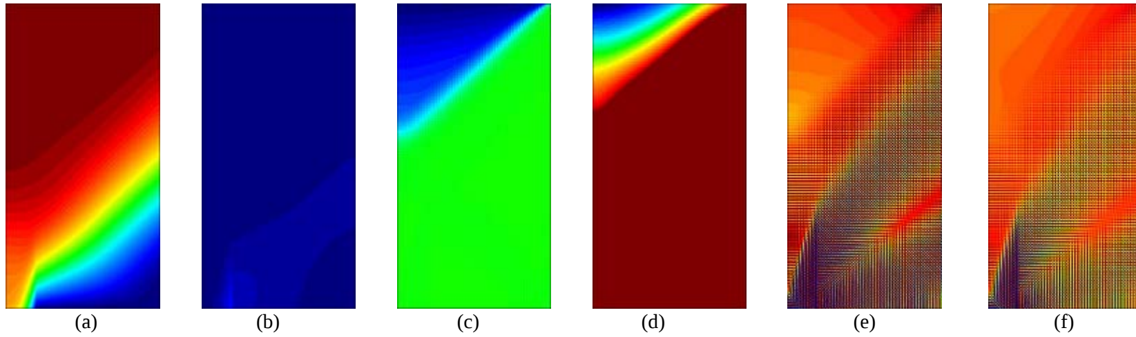
Figure 4.7 Contour fills for quadrilaterals irreducible u FE, von Mises: (a) Y-disp, (b) Equiv. plast. strain, (c) Lode angle, (d) J_2 stress, (e) Mean stress, (f) Y-stress
