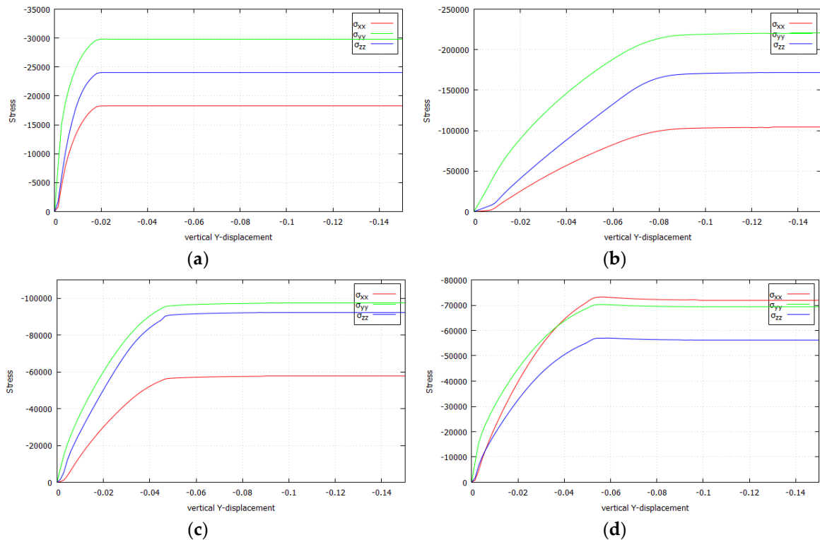
Figure 18. Stresses where the slide lines of Prandtl's Punch test (Plane Strain, \kappa = 3.0 ): (a) von Mises; (b) Parabolic Drucker-Prager; (c) Hoffman; (d) Tsai-Wu.
