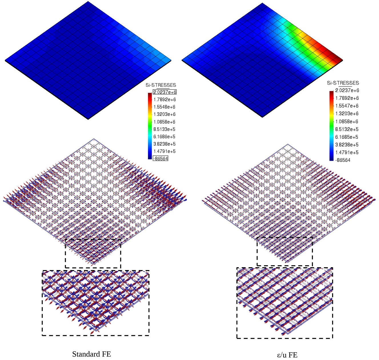
Fig. 39: Clamped square plate with 5 layers of orthotropic materials: Maximum principal stresses contour (top) and vectors (bottom) for standard (left) and \epsilon/u FEs (right) in a regular mesh of 16 elements per side.
