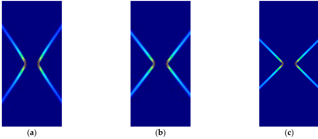
Figure 14. Strip under vertical plane strain tension (Cohesive-frictional models, \kappa = 3.0 ): (a) Parabolic Drucker-Prager; (b) Hoffman; (c) Tsai-Wu.
