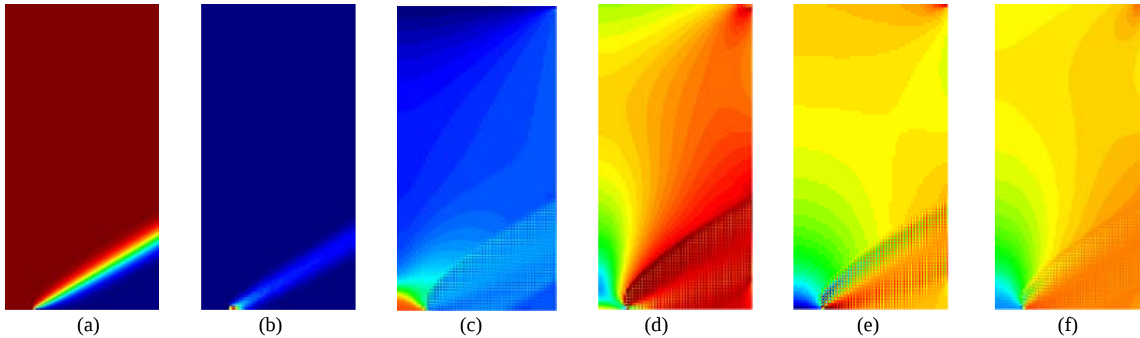
Figure 4.14 Contour fills for quads \bar{B} FE, Drucker-Prager: (a) Y-disp, (b) Equiv. plast. strain, (c) Lode angle, (d) J_2 stress, (e) Mean stress, (f) Y-stress
