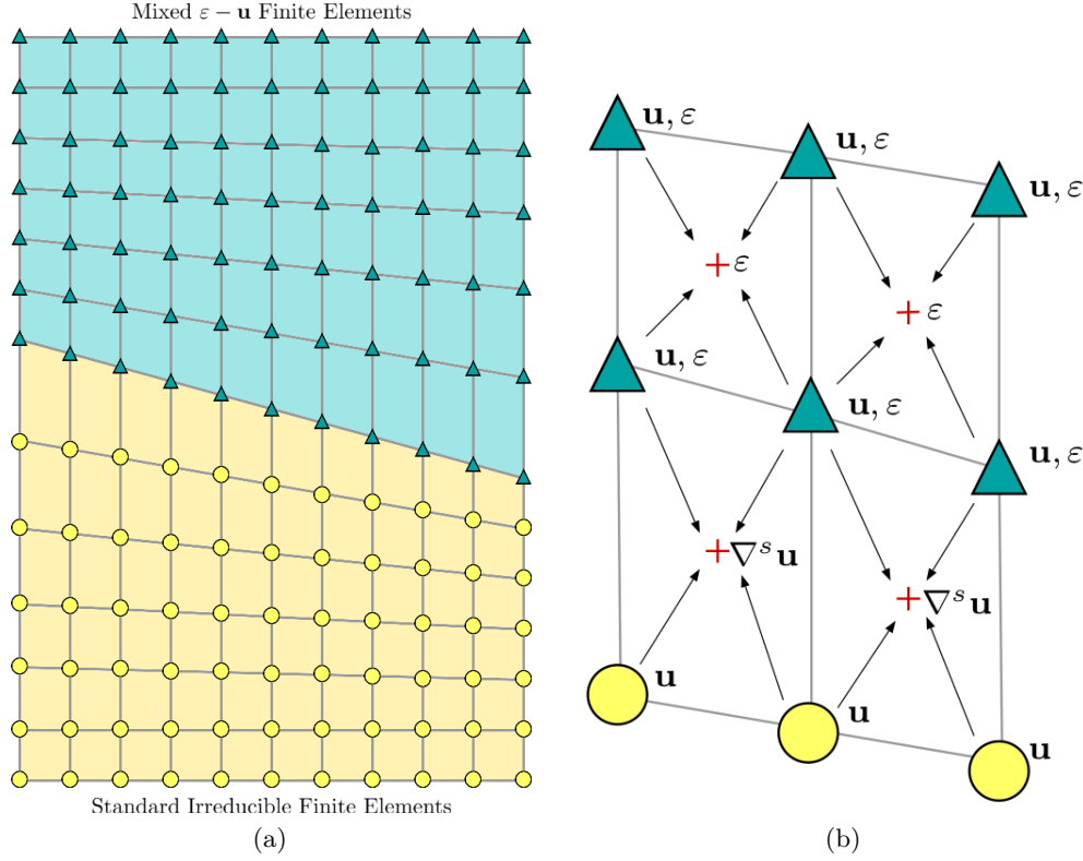
Figure 3.1: FE mesh with combined standard and mixed formulations. Turquoise color represents the mixed \epsilon - \mathbf{u} elements whereas yellow represents the displacement-based ones. The strain tensor at the Gauss points (symbolized with red crosses) is computed with the interpolation of nodal strain in the mixed formulation or the discrete symmetric gradient of displacements in the irreducible one.
