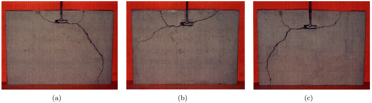
Figure 7: Asymmetric results for the second experimental setup (close bracing) [18]
