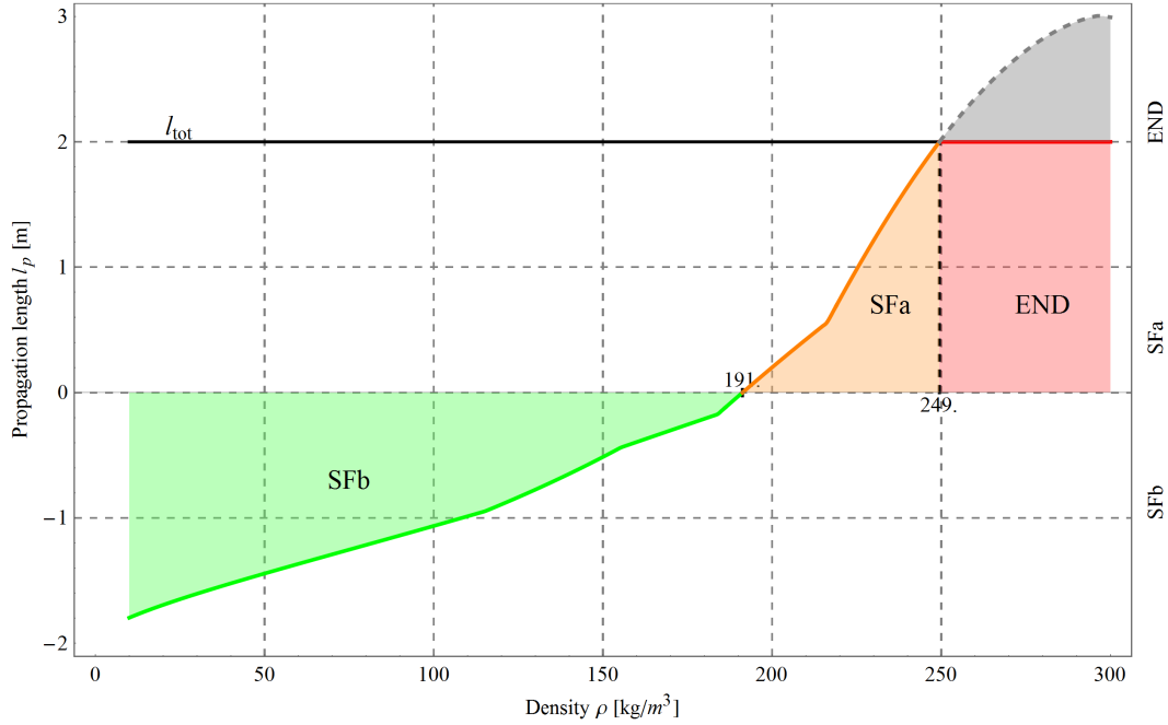
Figure 8.14: Signed propagation length with respect to the upper slab density for a 0.3 \times 0.3 \times 2 \text{ m}^3 specimen on a 35^\circ slope. The different test outcomes full propagation (END), slab fracture after propagation (SFa) and slab fracture before propagation (SFb) are highlighted on the plot with the respective limit values of density.
