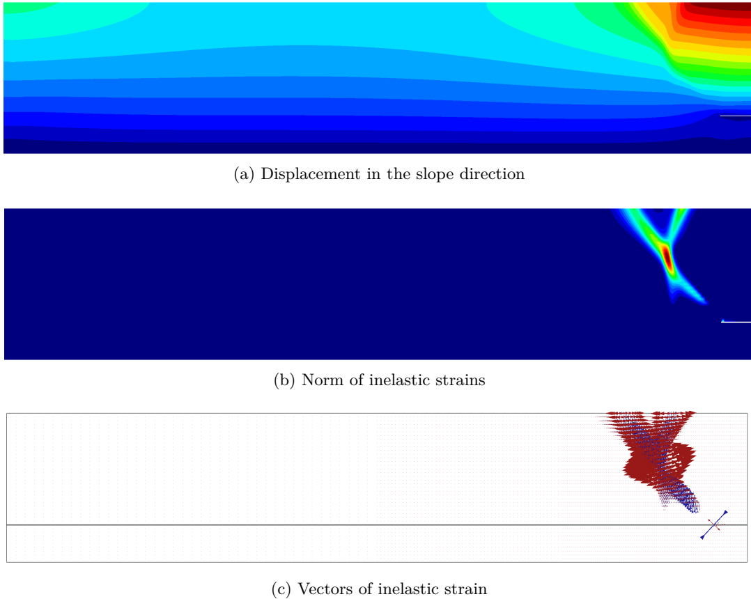
Figure 8.16: Numerical analysis for the slab fracture before propagation (SFb) case with a density of 180\text{kg/m}^3
