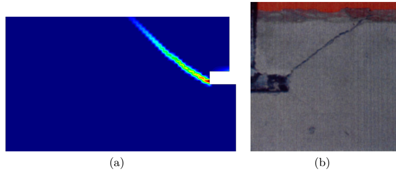
Figure 5.5: Comparing the symmetric pattern in the case of free horizontal sliding of the steel flange.
