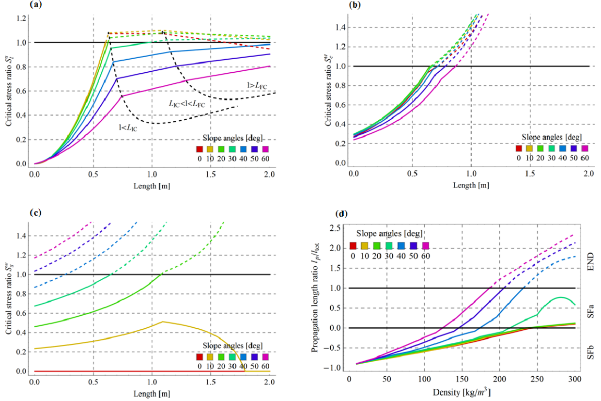
Figure 18: Model dependence to slope angles \psi (from 0^\circ to 60^\circ with 10^\circ steps): Figure (a), (b) and (c) show respectively the tensile stress in the upper slab, the compressive and the shear stresses in the weak layer plotted against length of saw cut; Figure (d) pictures the propagation length with respect to the upper slab density.
