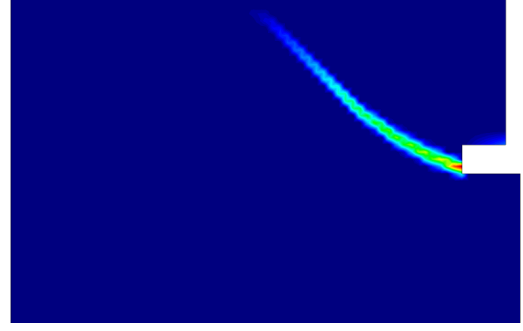
(b) \varepsilon/u FEM - No bracing
