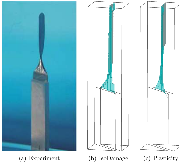
Figure 6: Experimental [10] and numerical ( \varepsilon - \mathbf{u} formulation) crack surface of the three point bending test on PMMA.
