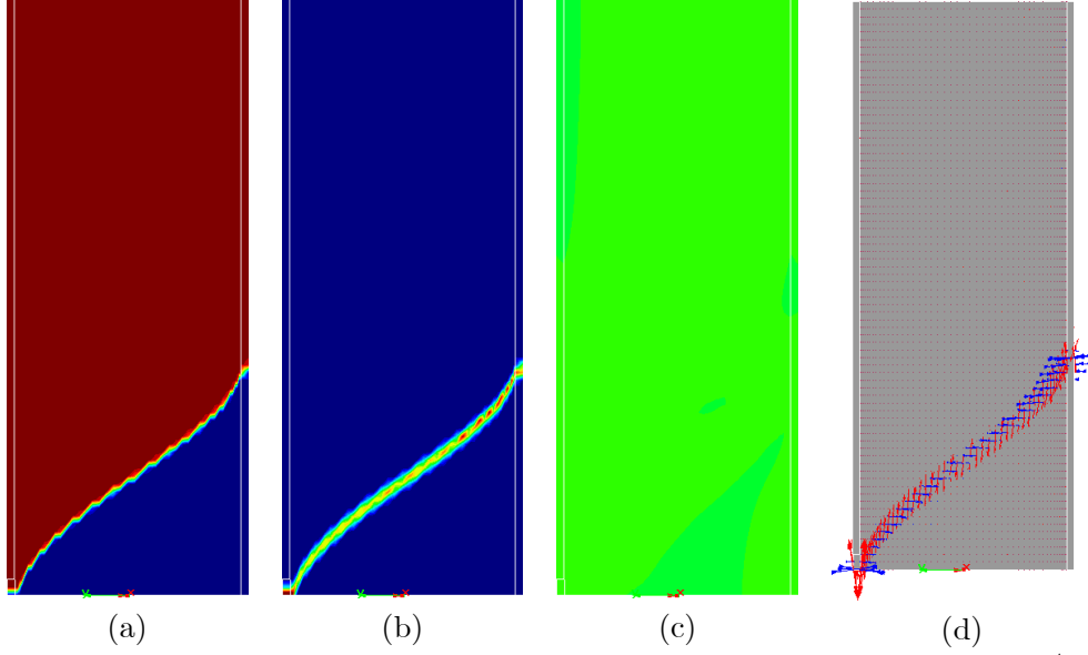
Figure 12: Results for simply perforated thin-walled cylinder with the mixed \boldsymbol{\varepsilon}/\mathbf{u} formulation. Contours for: (a) vertical displacement, (b) equivalent plastic strain, (c) pressure and (d) principal strain vectors
