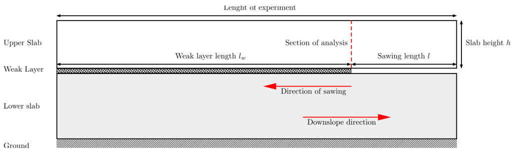
Figure 8.11: Side view sketch of the modeled Propagation Saw Test
