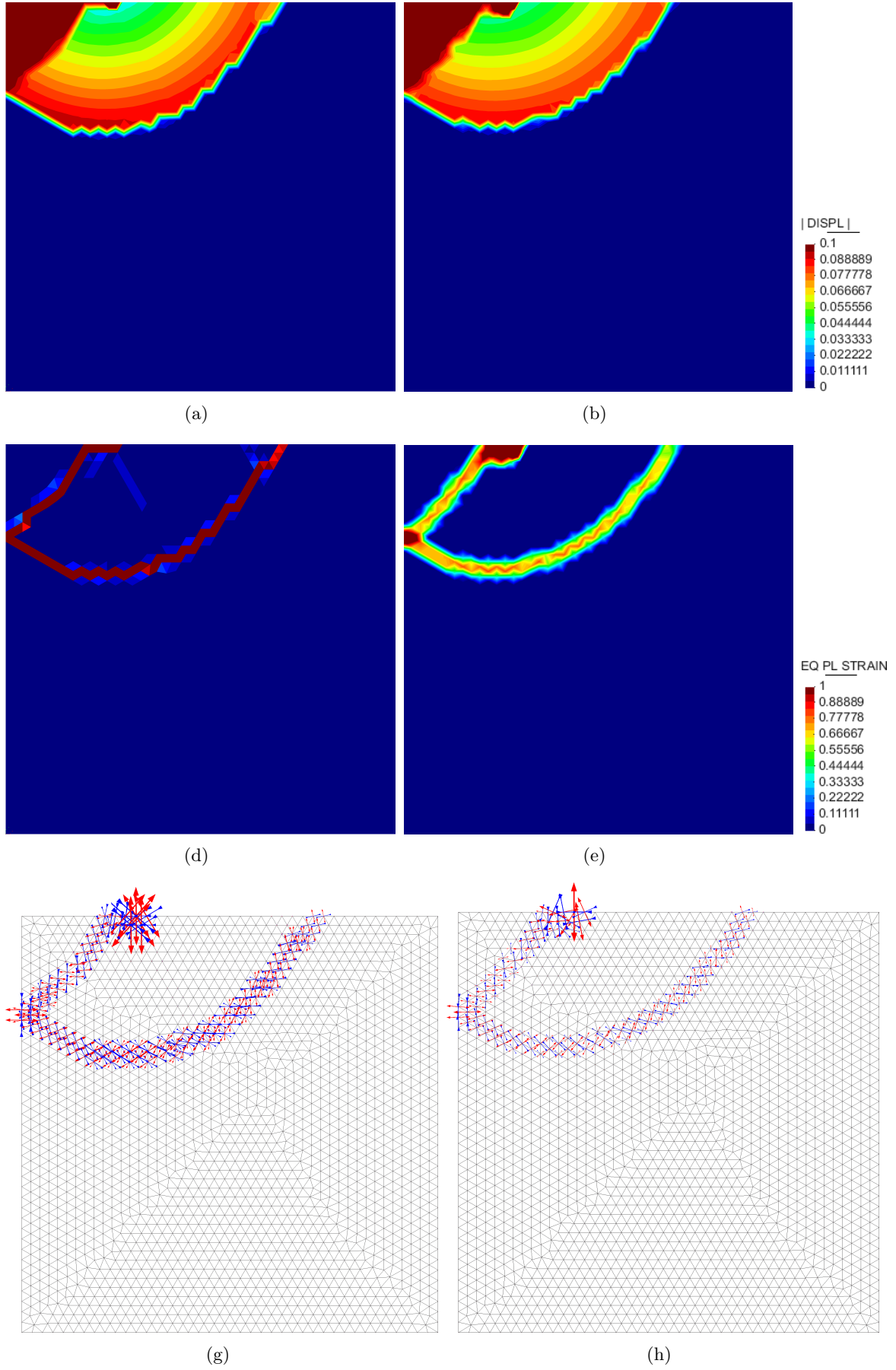
Figure 7: Results for Prandtl's punch problem: u/p (left column) and \varepsilon/u (right column). Contours of: total displacements (first row), equivalent plastic strain (second row), vectors of principal strains (third row).
