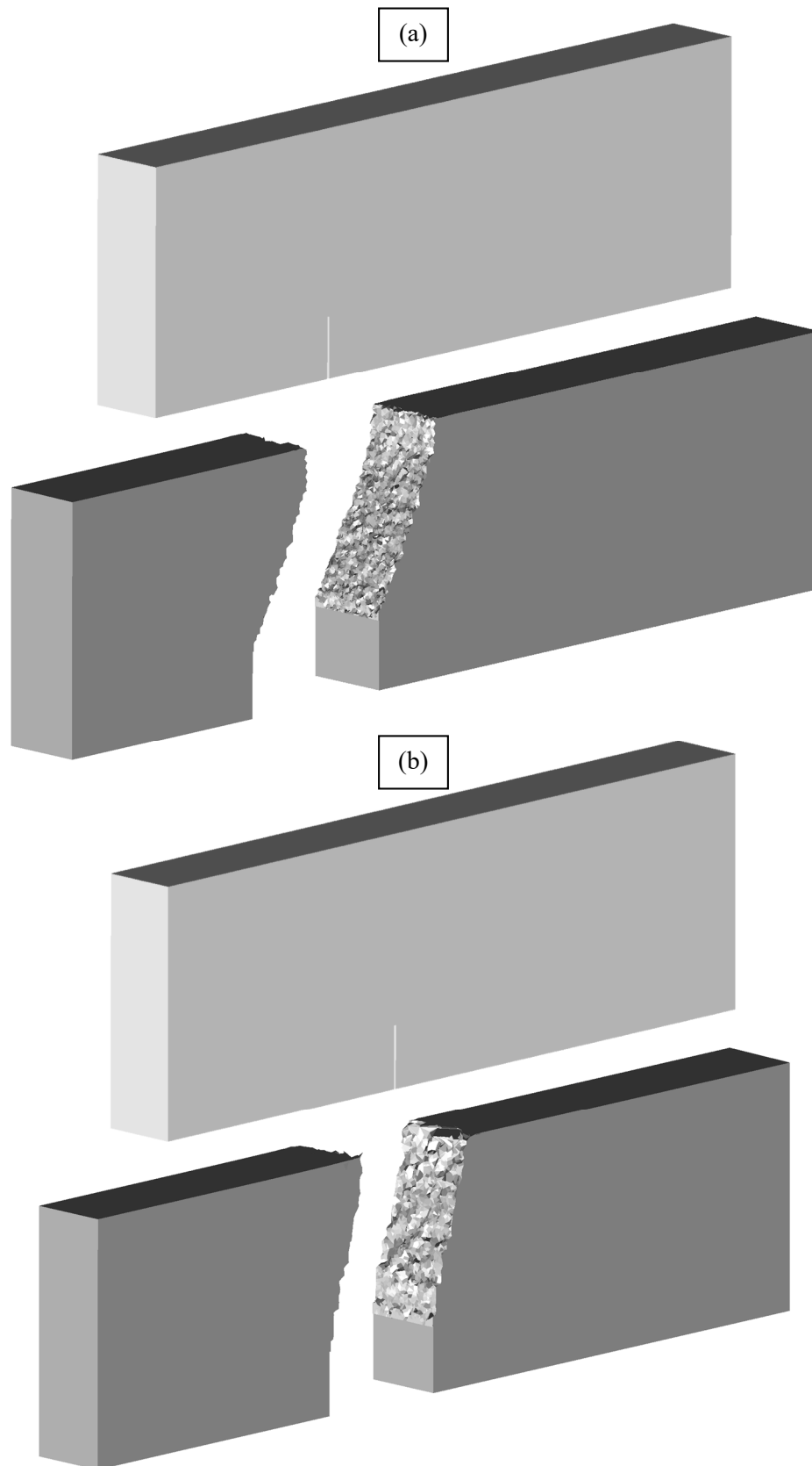
Figure 3.54: Computed crack surfaces of the Garcia-Alvarez beams, medium sizes, with eccentricities (a) 0.625D and (b) 0.3125D , with mixed FE
