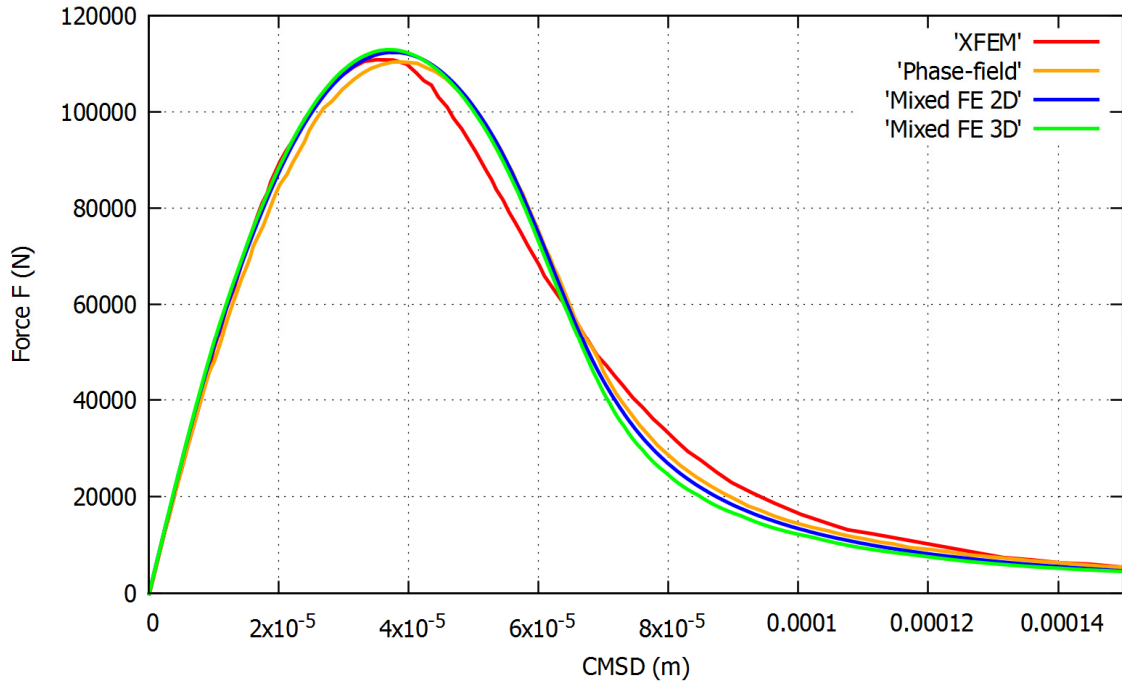
Figure 3.42: Comparison of the computed Force F vs. CMSD curves of the Arrea and Ingraffea beam in 2D and 3D
