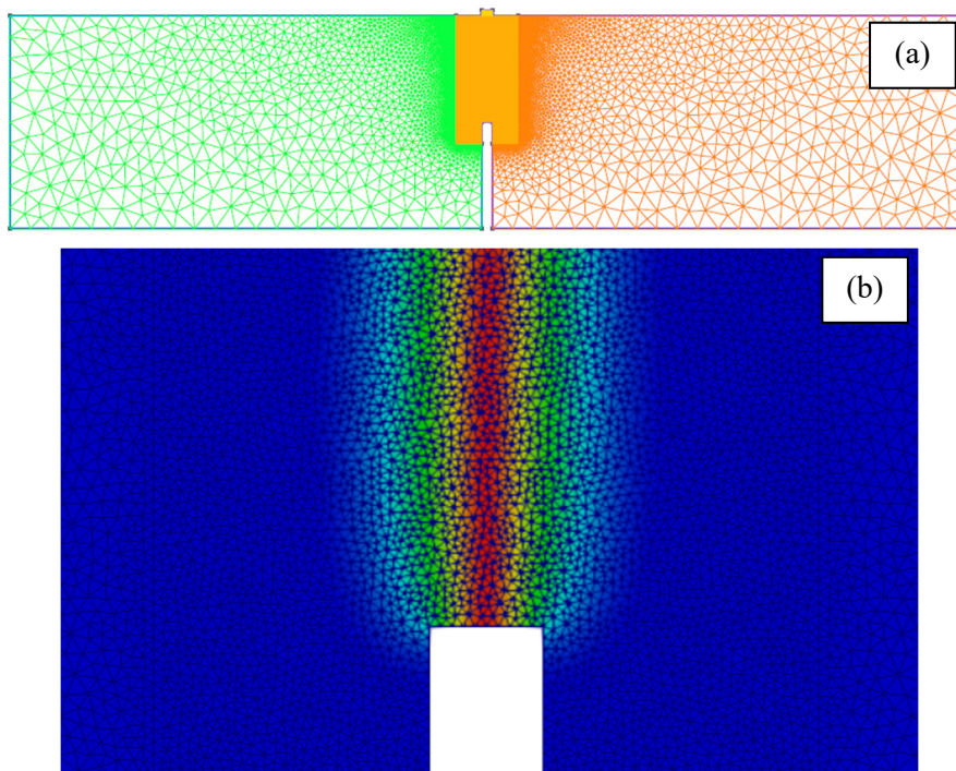
Figure 3.18: Mesh densities required in phase-field: three-point bending test of a notched beam: (a) model and (b) detail of the damage contour [63]
