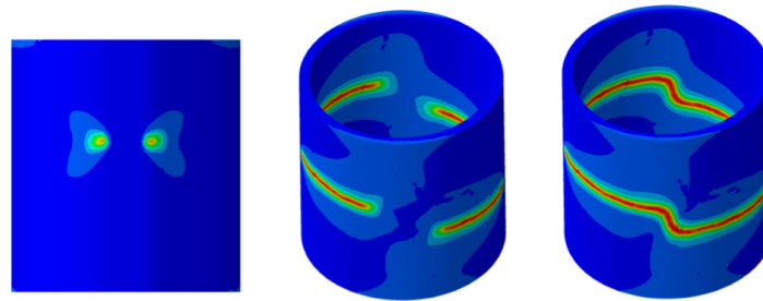
Figure 3.16: Crack propagation in a thick-walled cylinder computed with phase-field [260]
