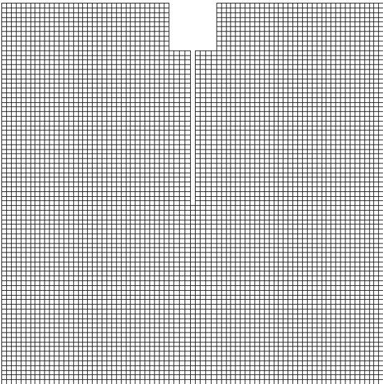
Figure 3.22: Mesh used for the wedge splitting test in the mixed FE simulations
