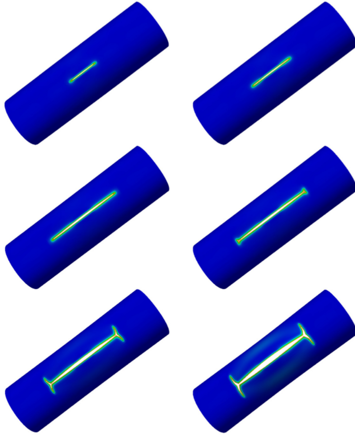
Figure 3.17: Cracking sequence of a hollow notched cylinder with tear straps under internal pressure computed with phase-field [268]
