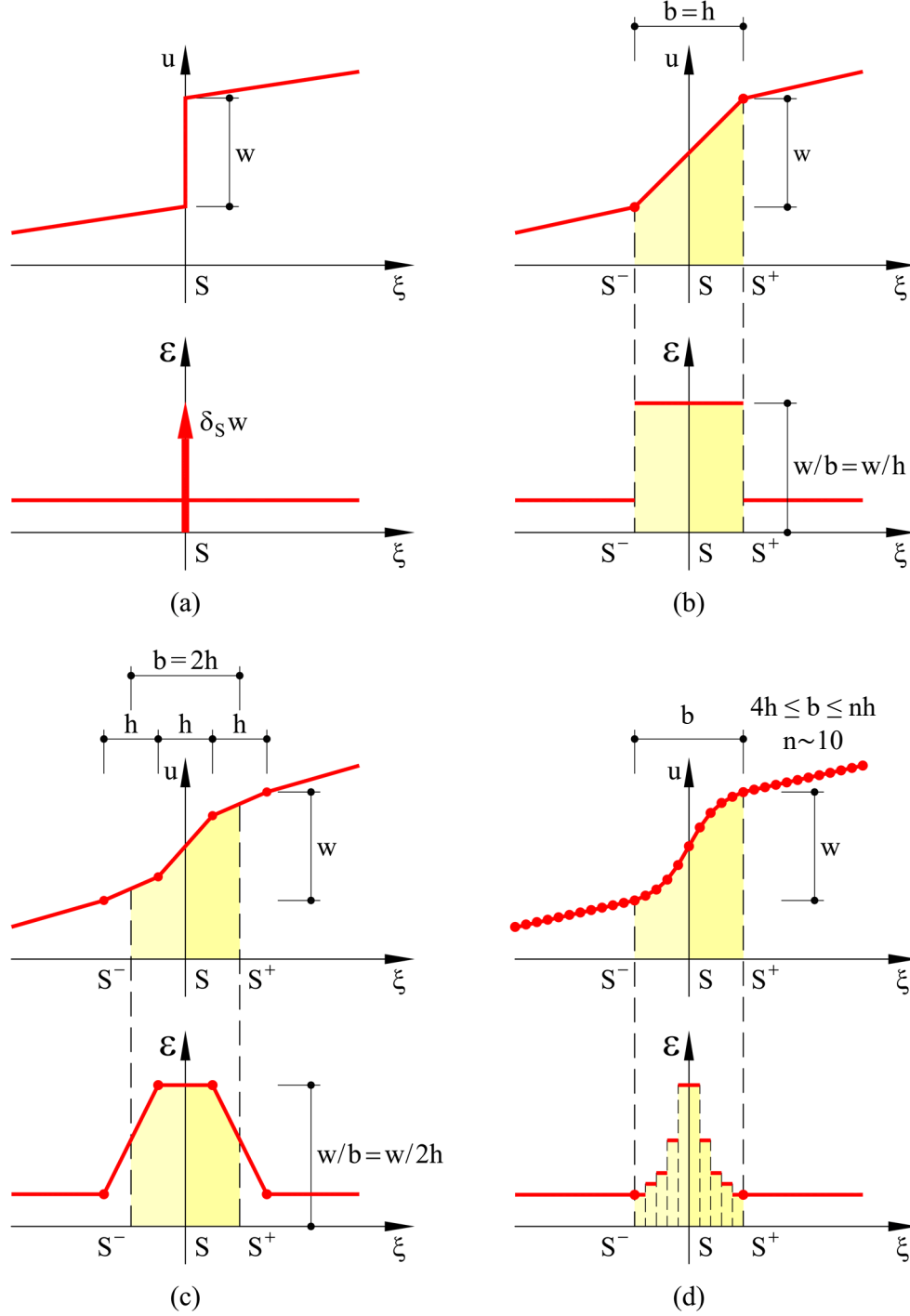
Figure 2.4: Depictions in the discrete setting of the (a) embedded model, (b) smeared crack model, (c) enhanced smeared crack model and (d) regularized model in terms of the displacement (up) and strain (bottom) fields
