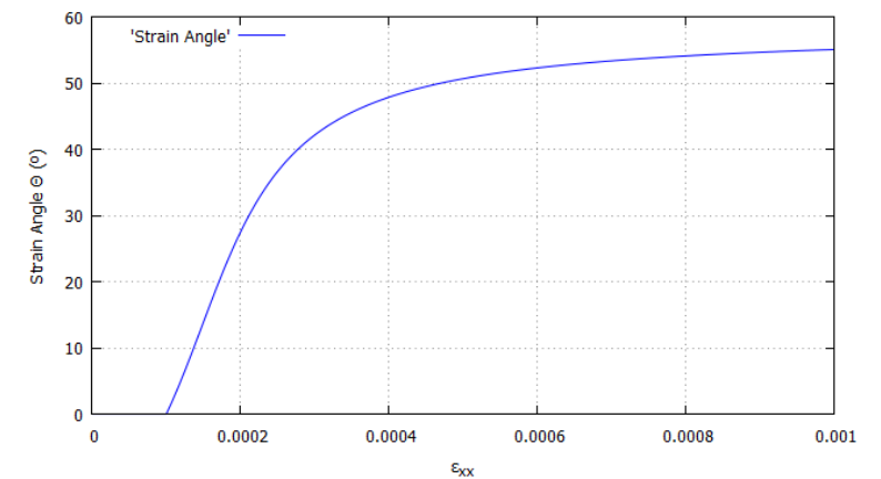
Figure 2. Evolution of the angle (degrees) of the maximum principal strain with respect to the X direction
