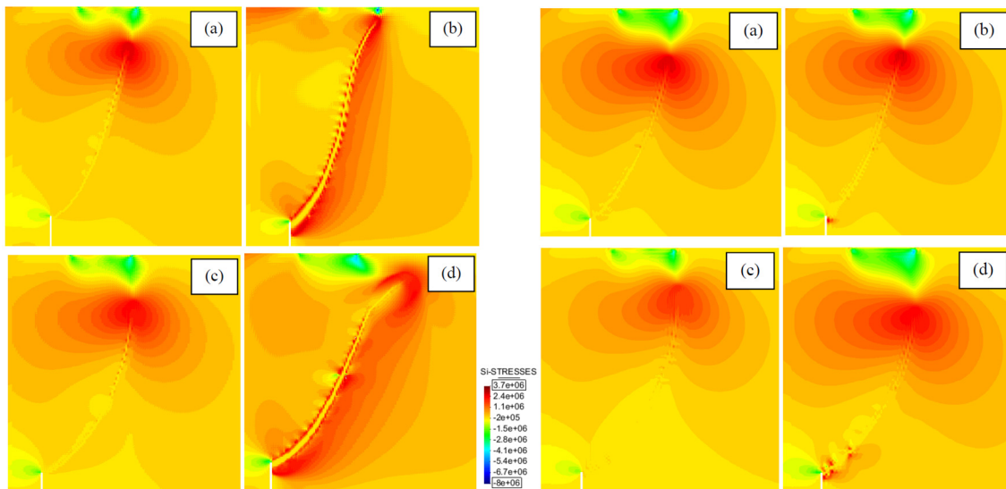
Figure 2.9. Contours of the major principal stress field in a mixed mode bending test computed with standard FE (left) and mixed FE (right) with different fracture criteria: (a) isotropic Rankine, (b) orthotropic Rankine, (c) isotropic Drucker-Prager and (d) orthotropic Drucker-Prager [32]
