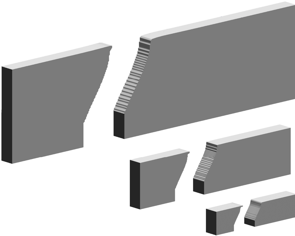
Figure 21. Computed crack surfaces of the mixed-mode fractured beams with eccentricity 0.625D for the three sizes of the series
