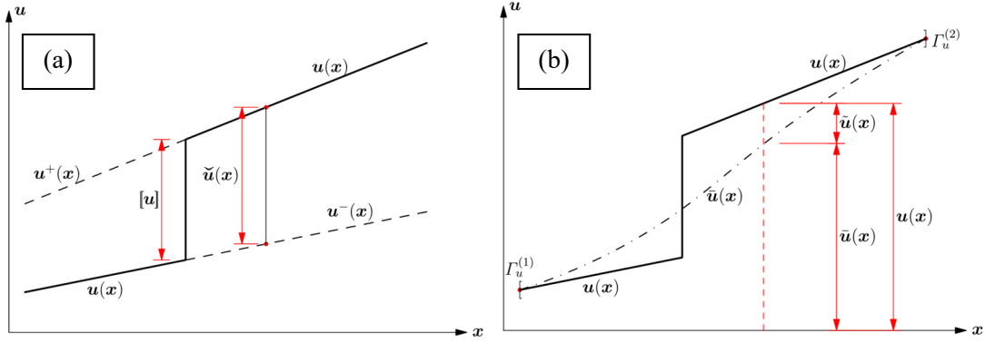
Figure 3.1: Strong discontinuity representing the crack in the continuous setting in Is-XFEM [75]
