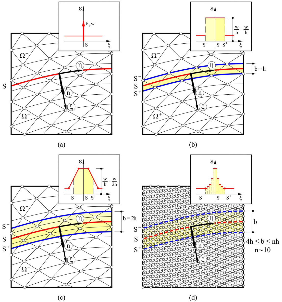
Figure 2.3: Depictions in the discrete setting of the (a) embedded model, (b) smeared crack model, (c) enhanced smeared crack model and (d) regularized model
