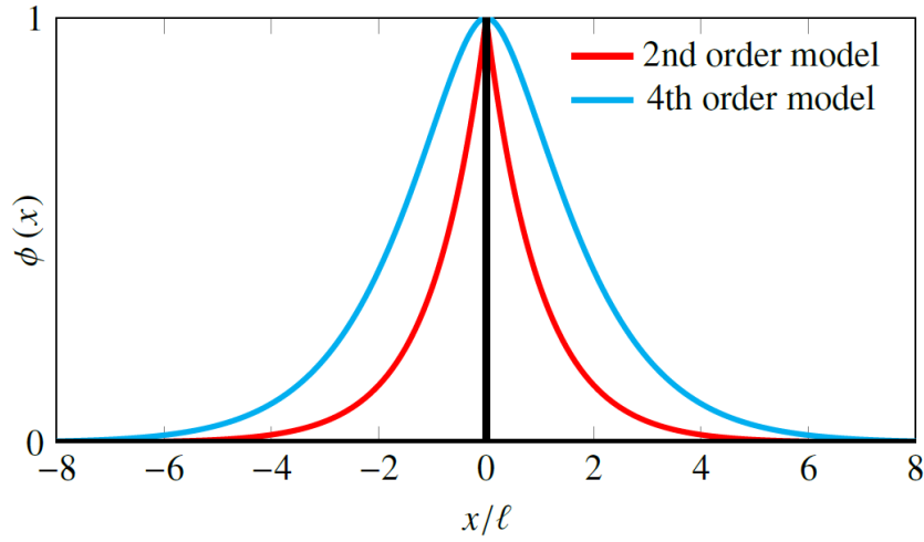
Figure 3.11: Damage profile of the 2 nd and 4 th order phase-field model [257], with \phi(x) being the phase-field variable identified with the damage d(x) and b = 2l
