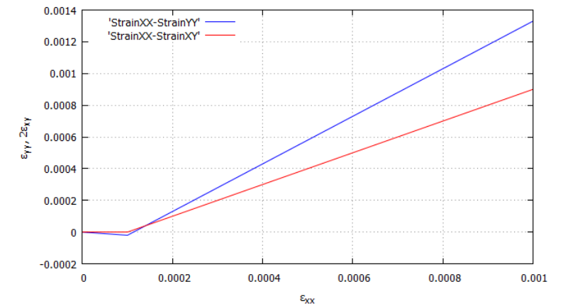
Figure 1. Imposed \epsilon_{xx} , \epsilon_{yy} and \epsilon_{xy} during Willam's test
