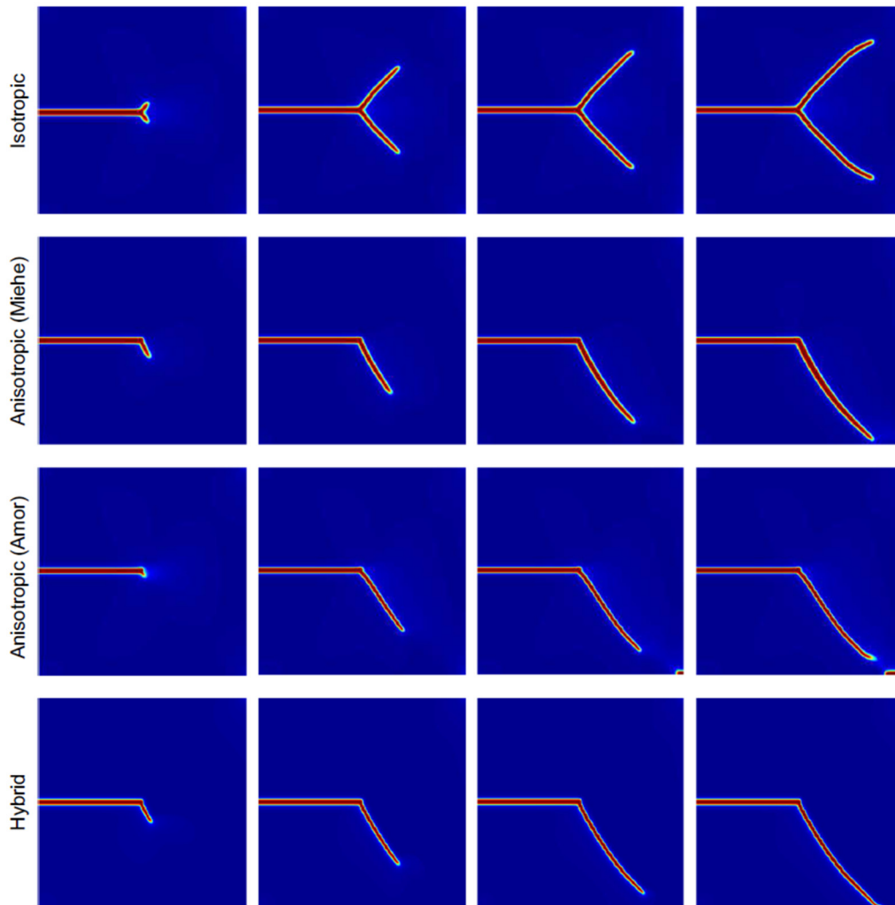
Figure 3.14: Comparison of damage contours obtained with isotropic, anisotropic and hybrid phase-field models, displayed in reference [259]
