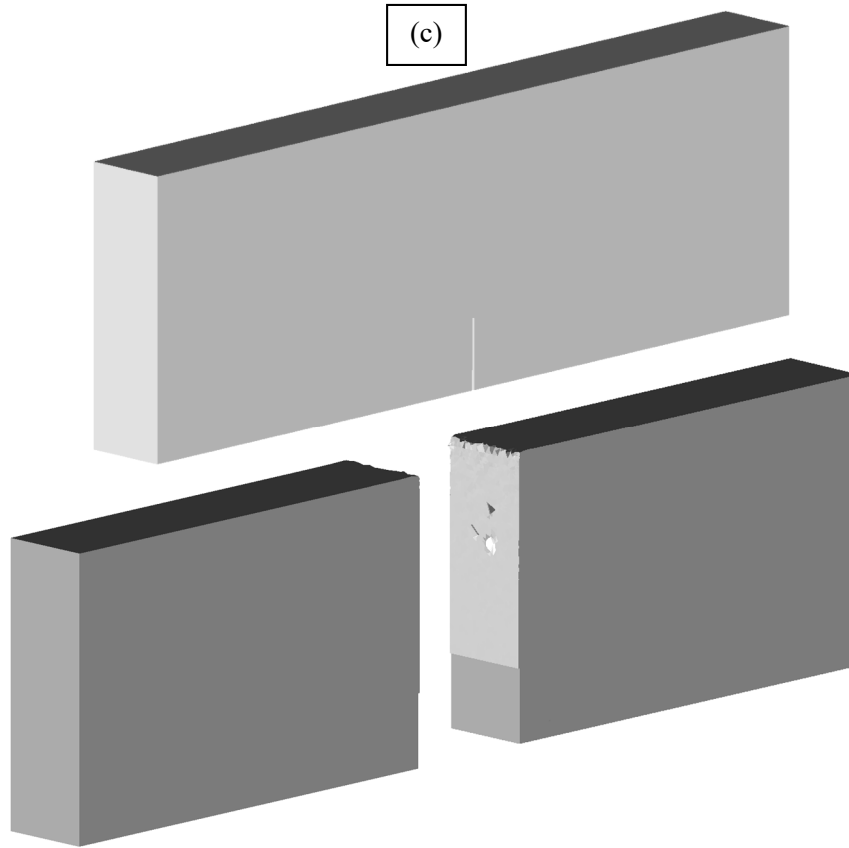
Figure 3.55: Computed crack surface of the Garcia-Alvarez beams, medium sizes, with eccentricity (c) 0.0D , with mixed FE
