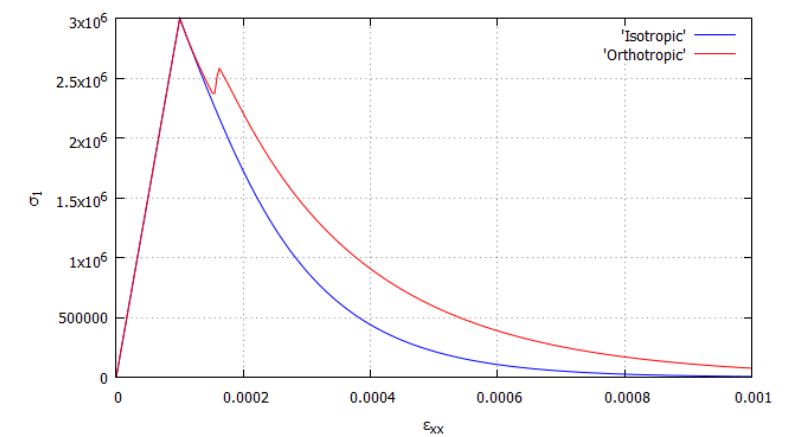
Figure 3. Computed maximum principal stress in Willam's test
