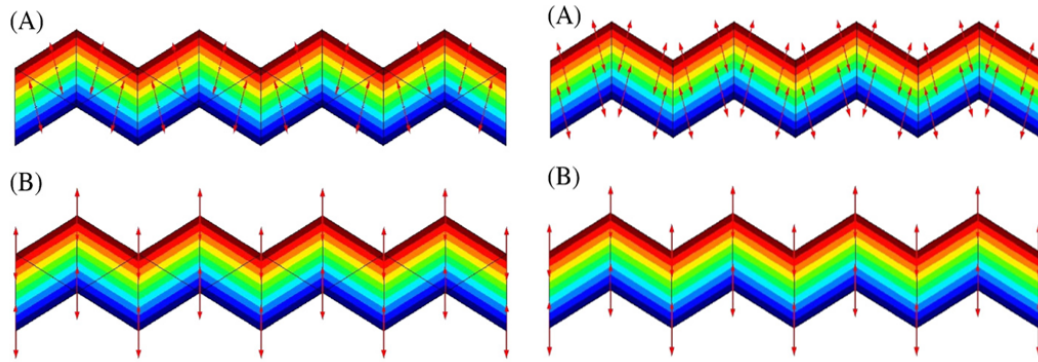
Figure 2.8: Standard (A) and mixed FEM (B) representation of separation modes in linear triangles (left) and quadrilaterals (right) [27]
