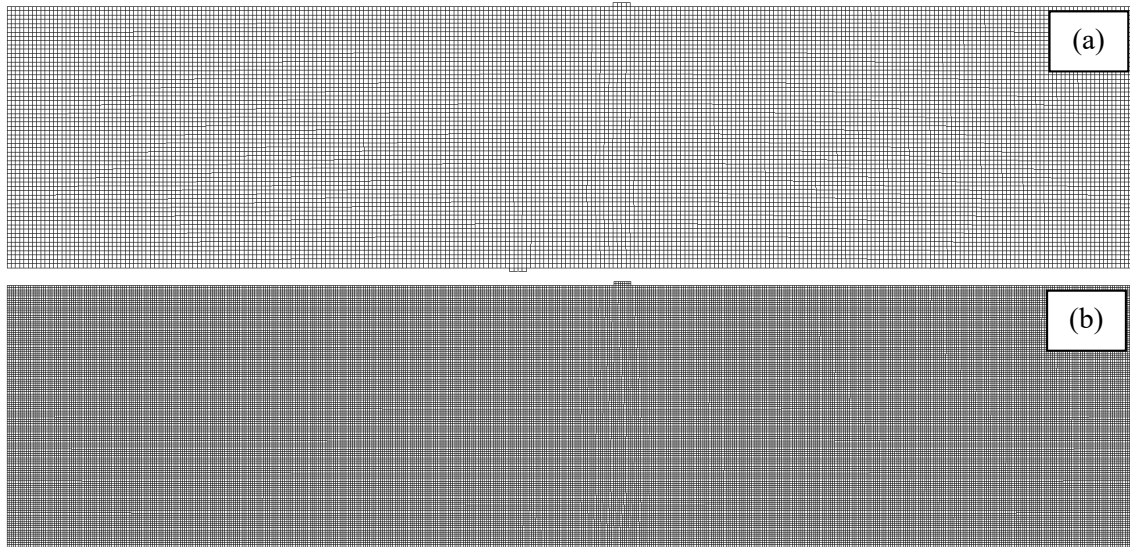
Figure 3.31: Meshes used for the Arrea and Ingraffea test in the mixed FE simulation with (a) h = 5 mm and (b) h = 2.5 mm
