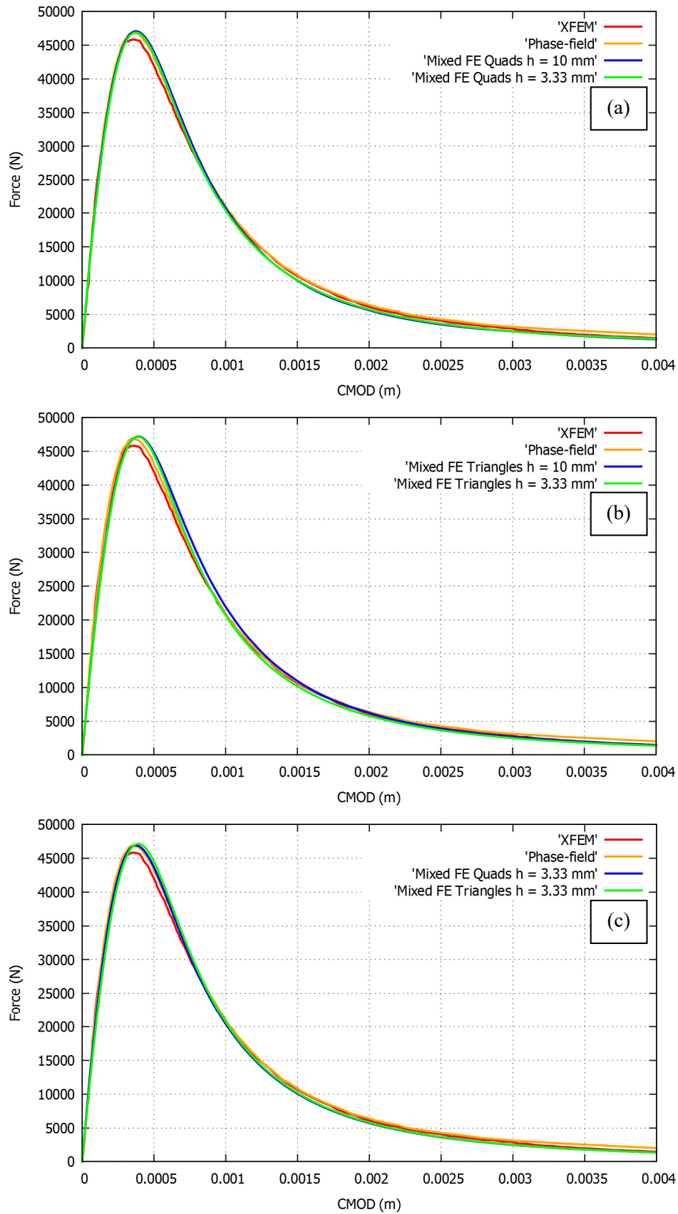
Figure 3.27: Mesh refinement analysis: Force-CMOD curve of the wedge splitting test for (a) quadrilateral elements, (b) for triangular elements and (c) quadrilateral vs. triangular FE comparison
