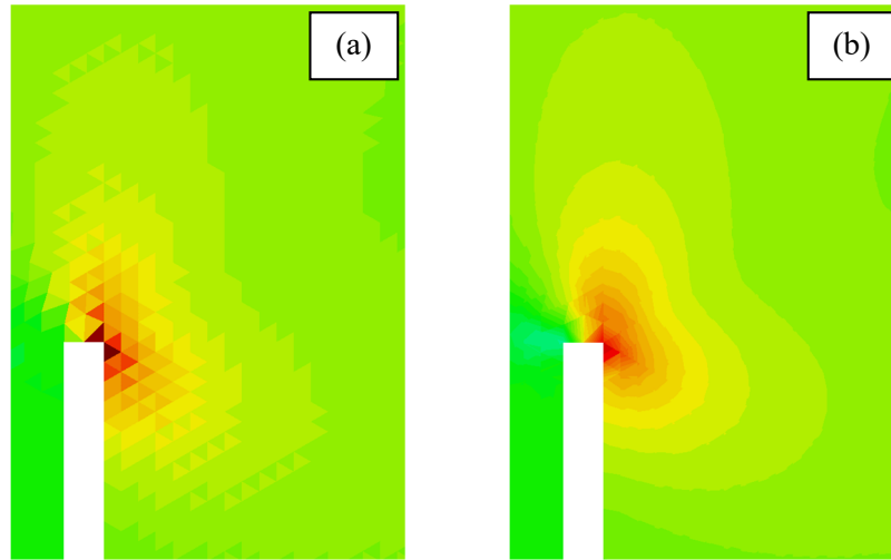
Figure 2.12: Contours of the major principal stress field around the tip of a notch in a mixed mode bending test computed using triangular elements with the (a) standard and (b) mixed formulations
