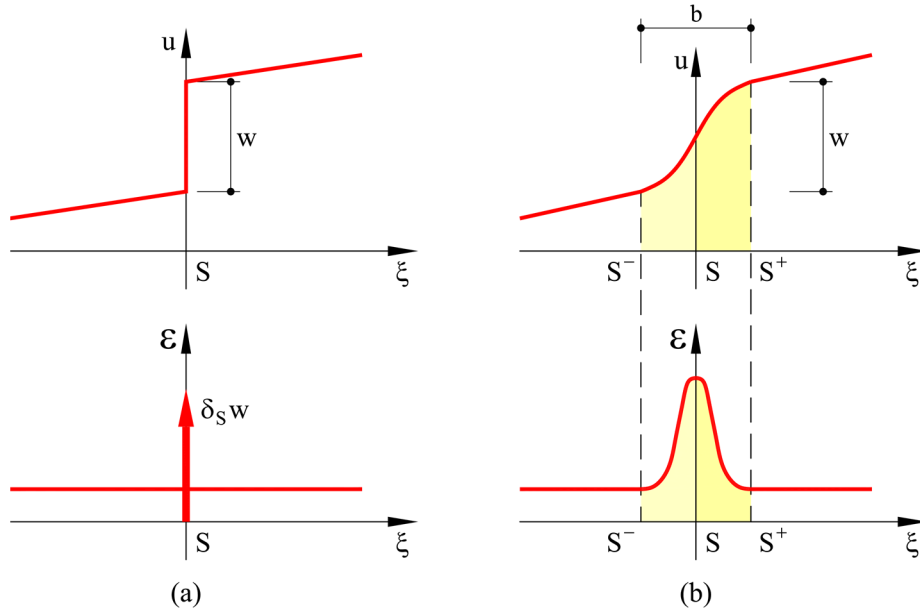
Figure 2.2: Depictions of (a) sharp and (b) regularized cracks in the continuous setting: displacement (up) and strain (bottom) fields
