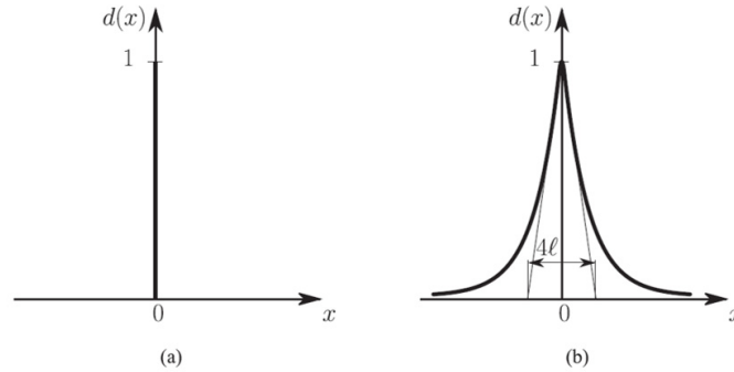
Figure 3.10: Representation of cracks using (a) embedded and (b) regularized models [253], with b = 4l
