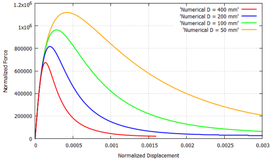
Figure 2.16: Force-displacement curves, normalized with size, of geometrically similar structures of varying sizes exhibiting size effect, computed with mixed FE [35]
